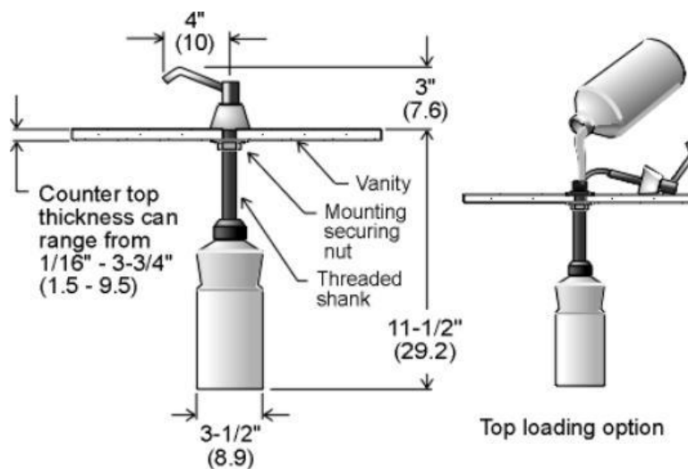
Part section, mounted view
