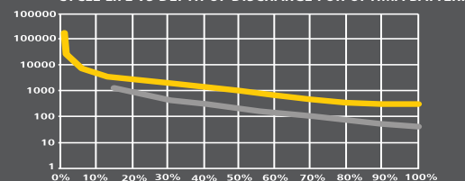
DEPTH OF DISCHARGE CYCLES TO 50% OF RATED CAPACITY
